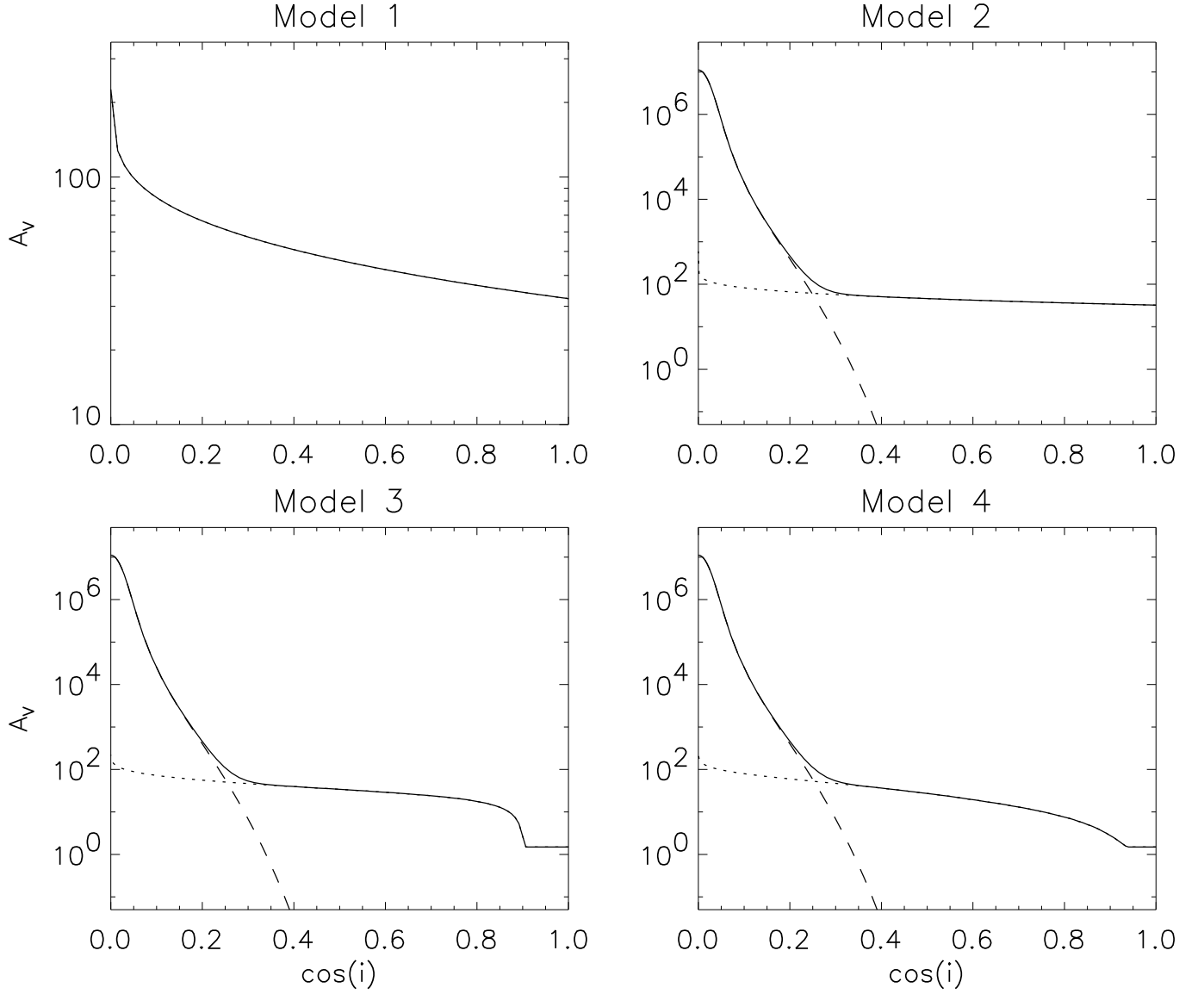
FIG. 3.— Optical extinction, A_V , from the central star through the envelope vs. inclination with respect to the polar axis, i . The dotted line shows extinction due to the envelope, the dashed line is that of the disk, and the solid is the sum. Note the large extinctions at edge-on inclinations for models with disks (Models 2-4).
