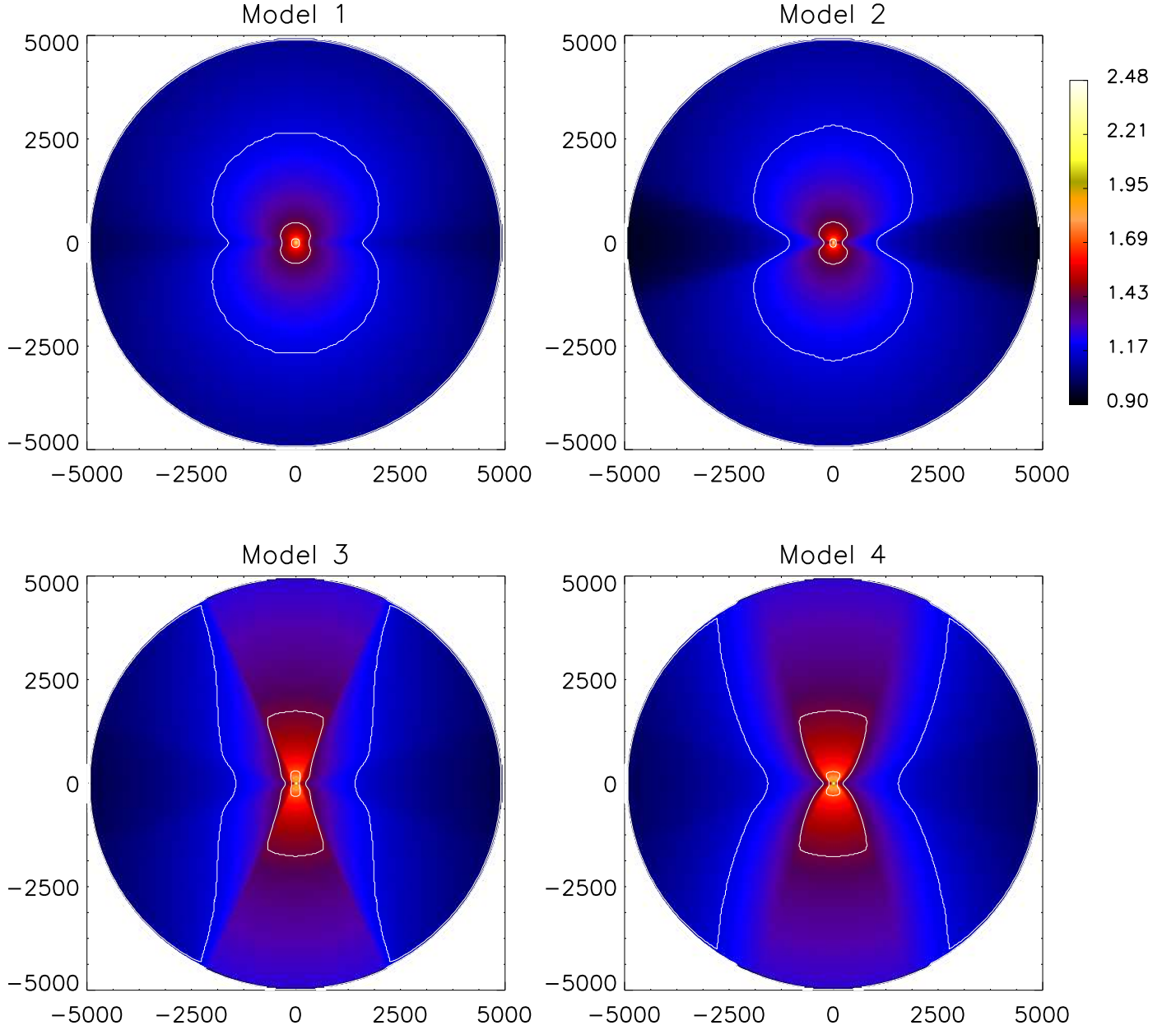
FIG. 4A.— Temperature plots for the 4 geometries. Images are scaled logarithmically with the color scale shown at the right. The contours correspond to the labelled values on the color bar (in units of \log(T) ). The plotted regions and temperature scales are (a) 5000 AU and T = 8 - 300^\circ\text{K} , (b) 300 AU, T = 22 - 1000^\circ\text{K} , and (c) 20 AU, T = 42 - 1600^\circ\text{K} .
