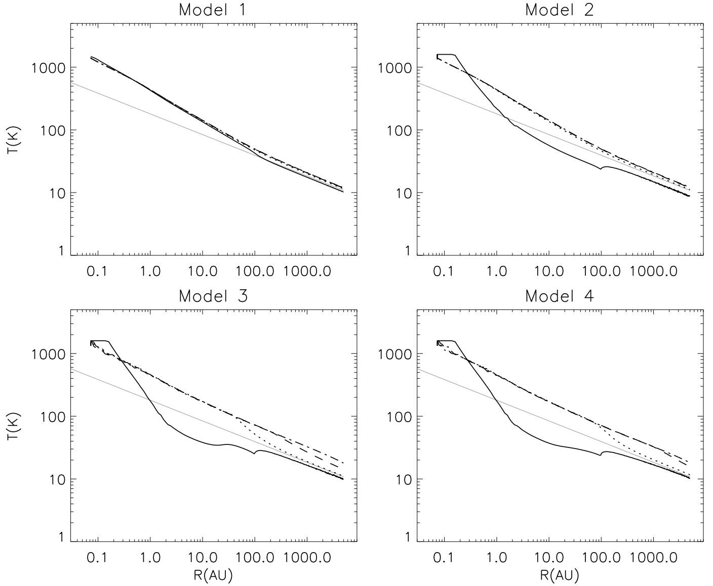
FIG. 5.— Temperature as a function of radius along four co-latitudes, \theta , with respect to the polar axis: \theta = 0 (dot-dashed line), \theta = 30 (dashed), \theta = 60 (dotted), and \theta = 90 (solid). The light grey line is a power law, T = 180 (r/1\text{AU})^{-0.33} \text{ K} .
