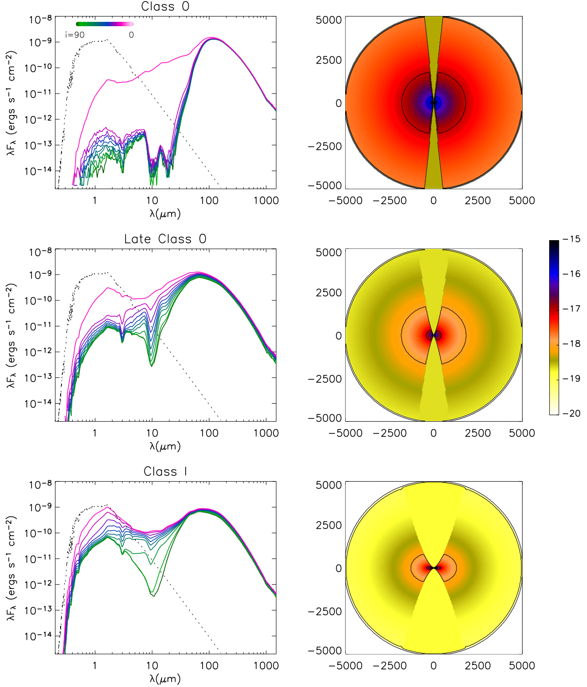
Fig. 3a.— SEDs (left) and densities (right) the 6 models. For the SED models, the colors indicate inclination, as shown in the top left panel: dark green is edge-on, and pink is pole-on. The density images are plotted to log scale, with the contours matching the tick marks in the color bar. The size range is noted in the axes in AU. Note that the Class II and III sources (disks) are much smaller than the envelope sources. (a) Class 0, late Class 0, & I (b) late Class I, Class II, & III.
