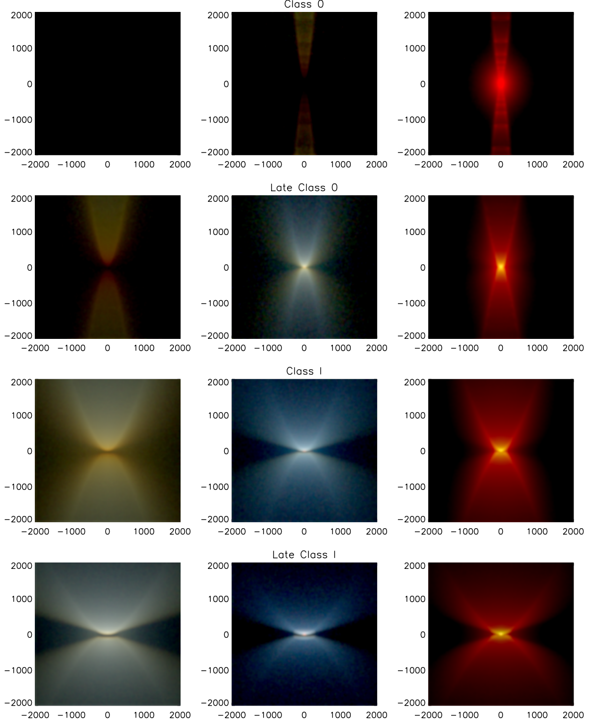
Fig. 11a.— 3-color composite images of the models. Left: 1.1, 1.6, and 2.05 \mu\text{m} ; middle: 3.6, average of 4.5 and 5.8, and 8.0 \mu\text{m} ; right: 8.0, 24, and 70 \mu\text{m} . The images are scaled logarithmically from the minimum intensity described in the text to 4 orders of magnitude above. The inclination is 80^\circ . The axis labels show the size of the image in AU. (a) Class 0, Late 0, I, and Late I models. (b) Class II and III models.
