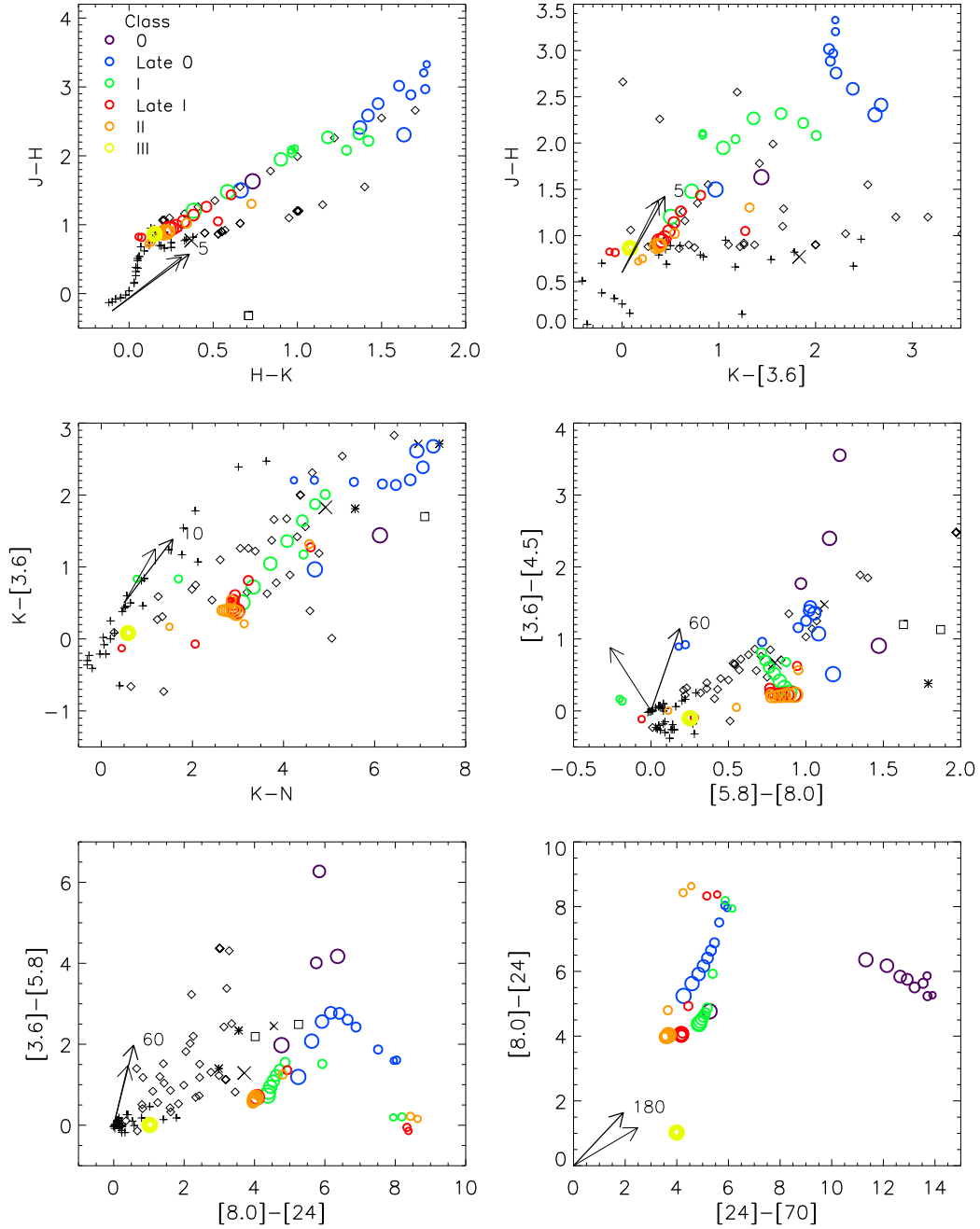
Fig. 7a.— Color-color plots. The legend in the top left panel shows the color correspondence with the evolutionary sequence. The symbol sizes vary with inclination with edge-on the smallest. Arrows show the reddening vectors for standard ISM dust (grey arrow) and dust more representative of dark clouds with r_v = 4 (our Envelope grains) (black arrow). The black symbols are predictions for other stellar types as follows—crosses: main sequence, red giant, supergiants; diamonds: AGB stars; squares: planetary nebulae; asterisks: reflection nebulae; small x: HII region; large X: T Tauri star. a) Aperture size is 1000 AU radius. b) Aperture size is 5000 AU radius.
