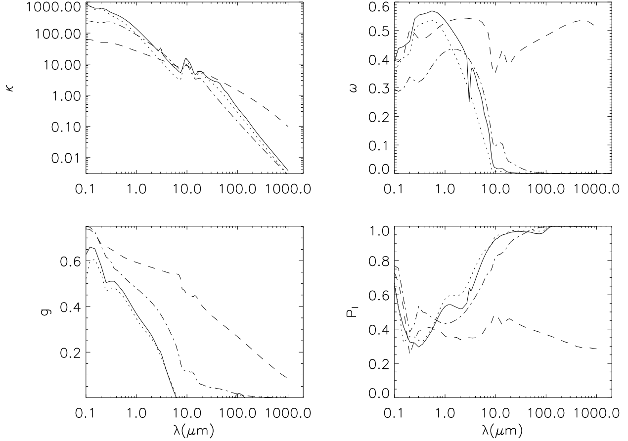
Fig. 2.— Dust properties of the 4 grain models. Opacity ( \kappa ) is shown in the top left panel, albedo ( \omega ) at top right, average cosine of scattering angle ( g ) is bottom left, maximum polarization ( P_l , typically at 90^\circ scattering angle) is bottom right. The four lines show the four grain models from Figure 1 as follows: Envelope, solid line; Outflow, dotted; Disk Midplane, dashed; Disk Atmosphere, dot-dashed.
