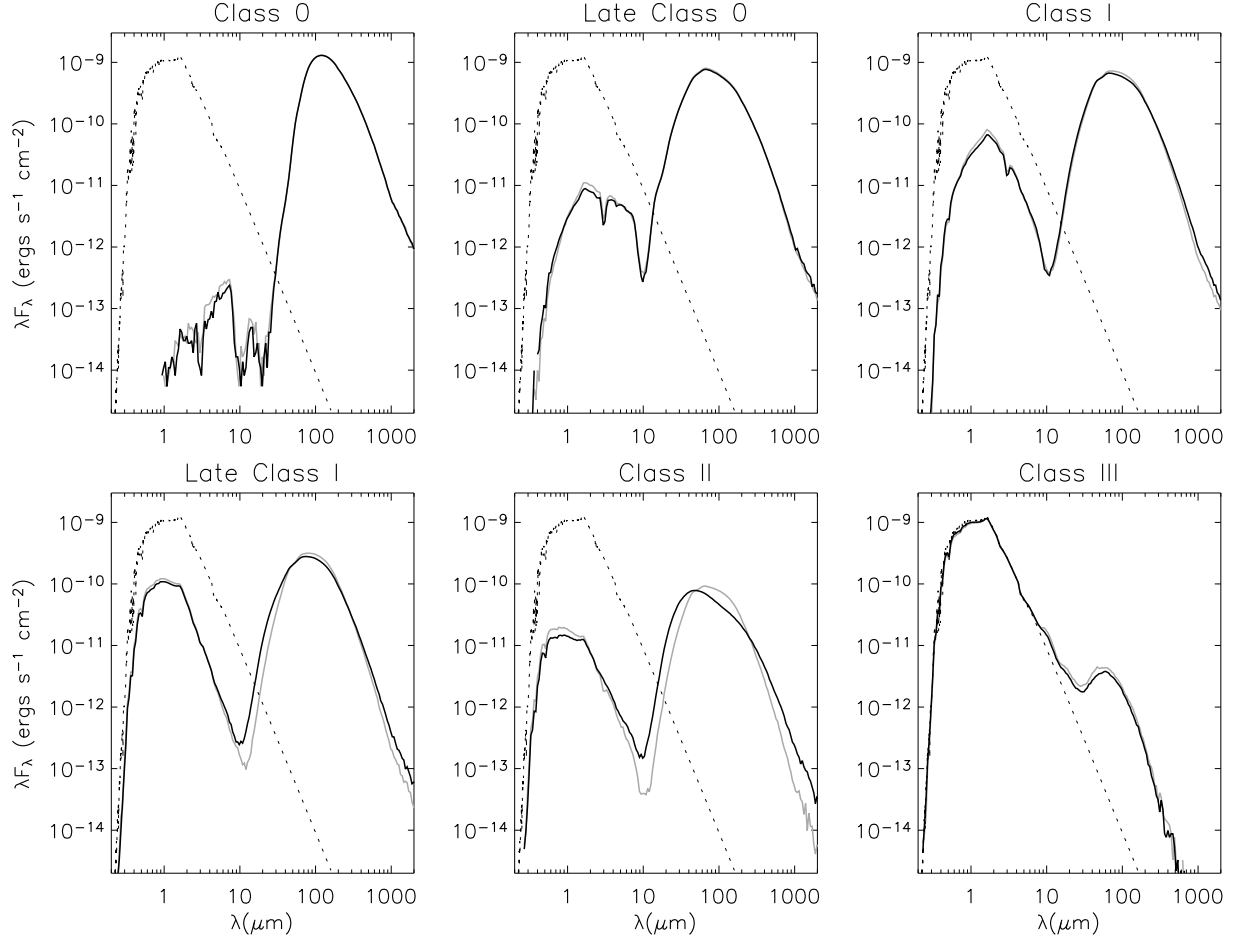
Fig. 6a.— Comparison of the SEDs produced from the different dust models. The black line plots the results from using different dust models for the four different regions (see Figure 1 and Table 3). The grey line shows results using the Envelope dust ( r_v = 4.3 ) throughout. (a) inclination is i=87 (edge-on) (b) inclination is i=56 (c) inclination is i=18 (pole-on)
