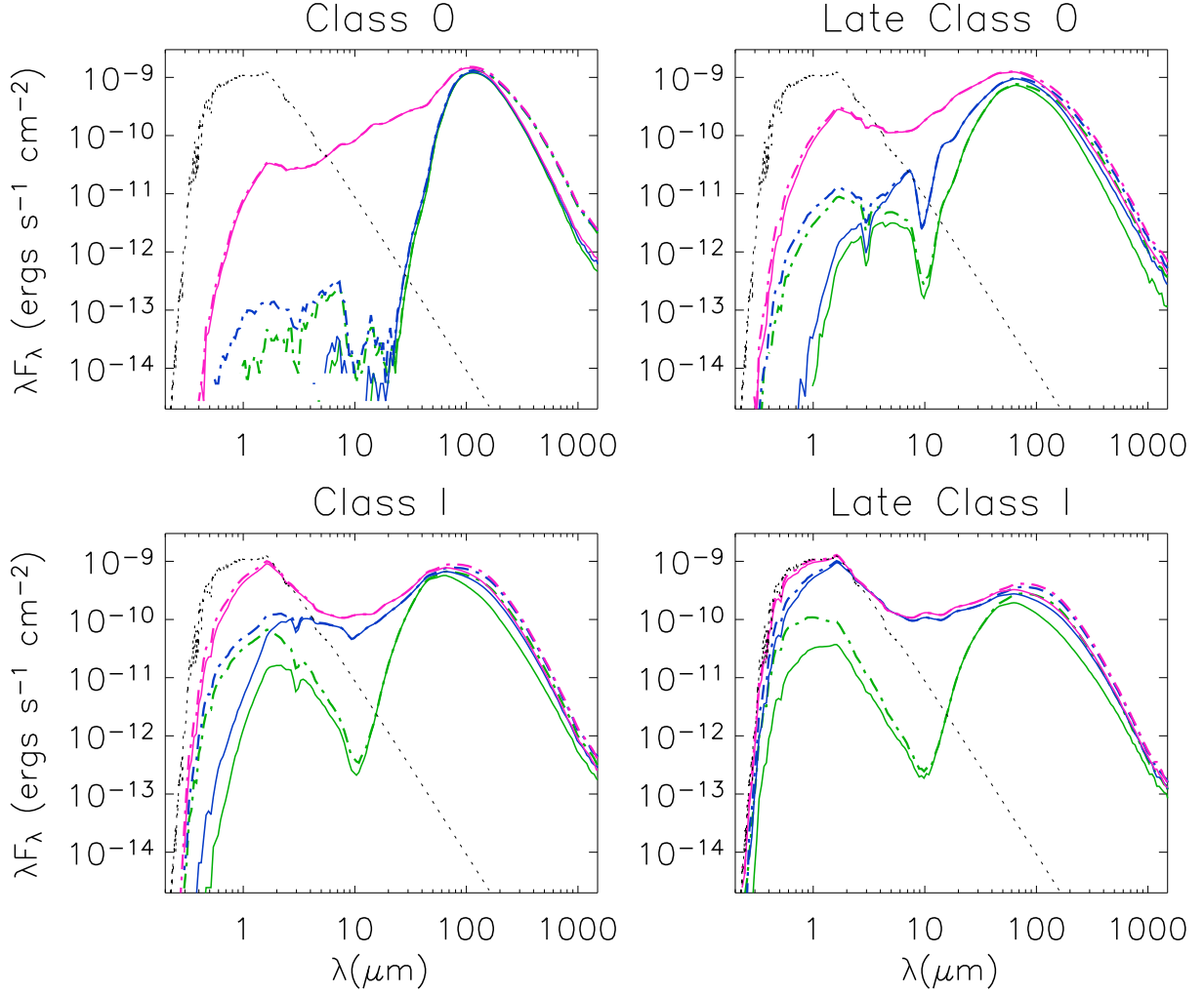
Fig. 4.— Comparison of SEDs computed in different aperture sizes for the sources with envelopes (Class 0-I). Small aperture results (1000 AU radius) are shown as solid lines; large aperture results (5000 AU radius) are dot-dashed. Three inclinations are plotted for each model ( i = 18, 56, 87^\circ ) as separate colors (pink, blue, green respectively)
