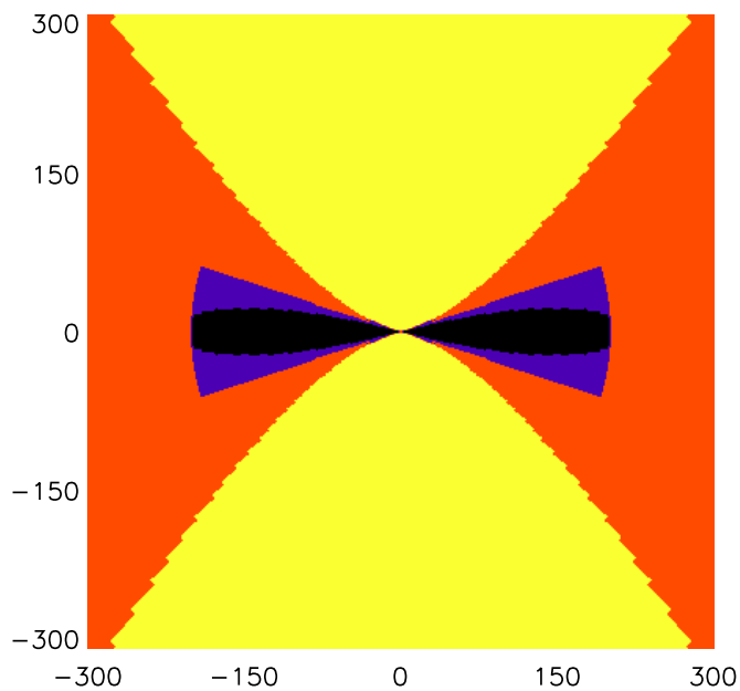
Fig. 1.— The inner region of the grid (300 AU) showing the regions where the different grain models are used. Grid cells colored black have the Disk Midplane grains (from Wood et al. 2002); blue cells have the Disk Atmosphere grains (from Coter et al. 2001); red cells have the Envelope grains (Paper I); and yellow cells have the Outflow grains (ISM grains from Kim, Martin, & Hendry 1994).
