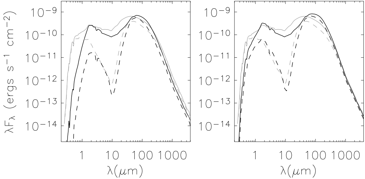
Fig. 5.— SEDs at selected inclinations for a Class I source (black) and Class II source (grey). The luminosity of the Class II source is scaled up by a factor of 5. The Class I results are shown for an aperture of 1000 AU at left, and 5000 AU at right. The dashed lines show inclinations of i = 87^\circ for the Class I and II sources. The solid lines show inclinations of i = 41^\circ for the Class I source and i = 75^\circ for the Class II source.
