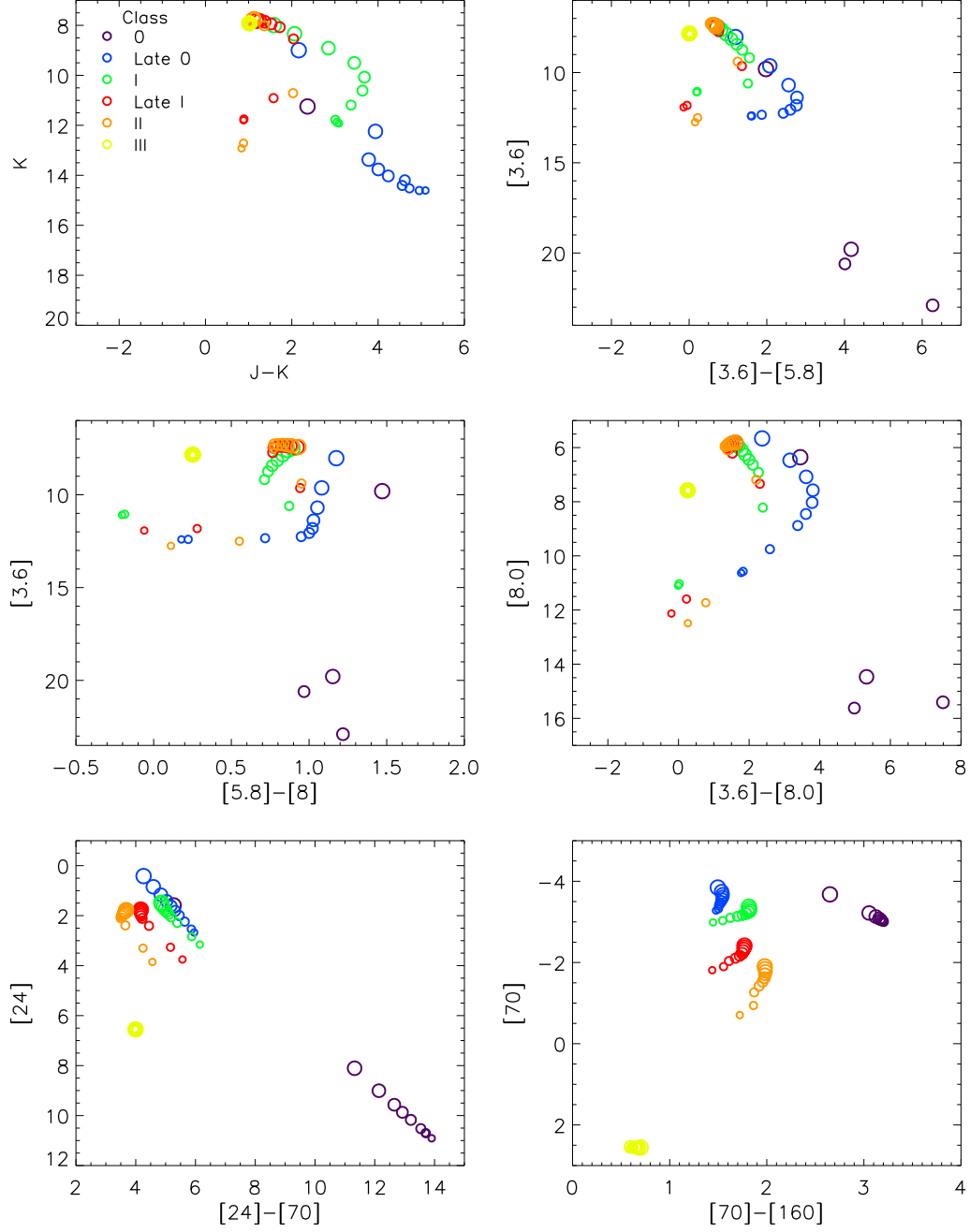
Fig. 8a.— Color-magnitude plots. The legend in the top left panel shows the color correspondence with the evolutionary sequence. The symbol sizes vary with inclination with edge-on the smallest. a) Aperture size is 1000 AU radius. b) Aperture size is 5000 AU radius.
