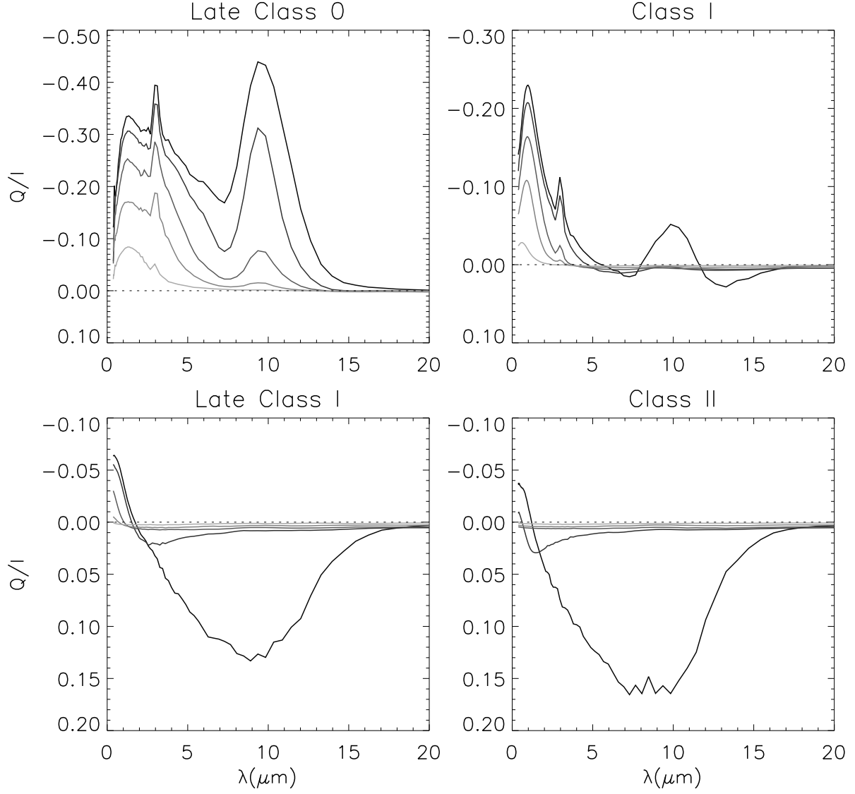
Fig. 9.— Polarization. Five inclinations are plotted from \cos i = 0.05 to 0.85 in intervals of 0.2 . The lines are lighter grey at lower inclinations (more pole-on).
