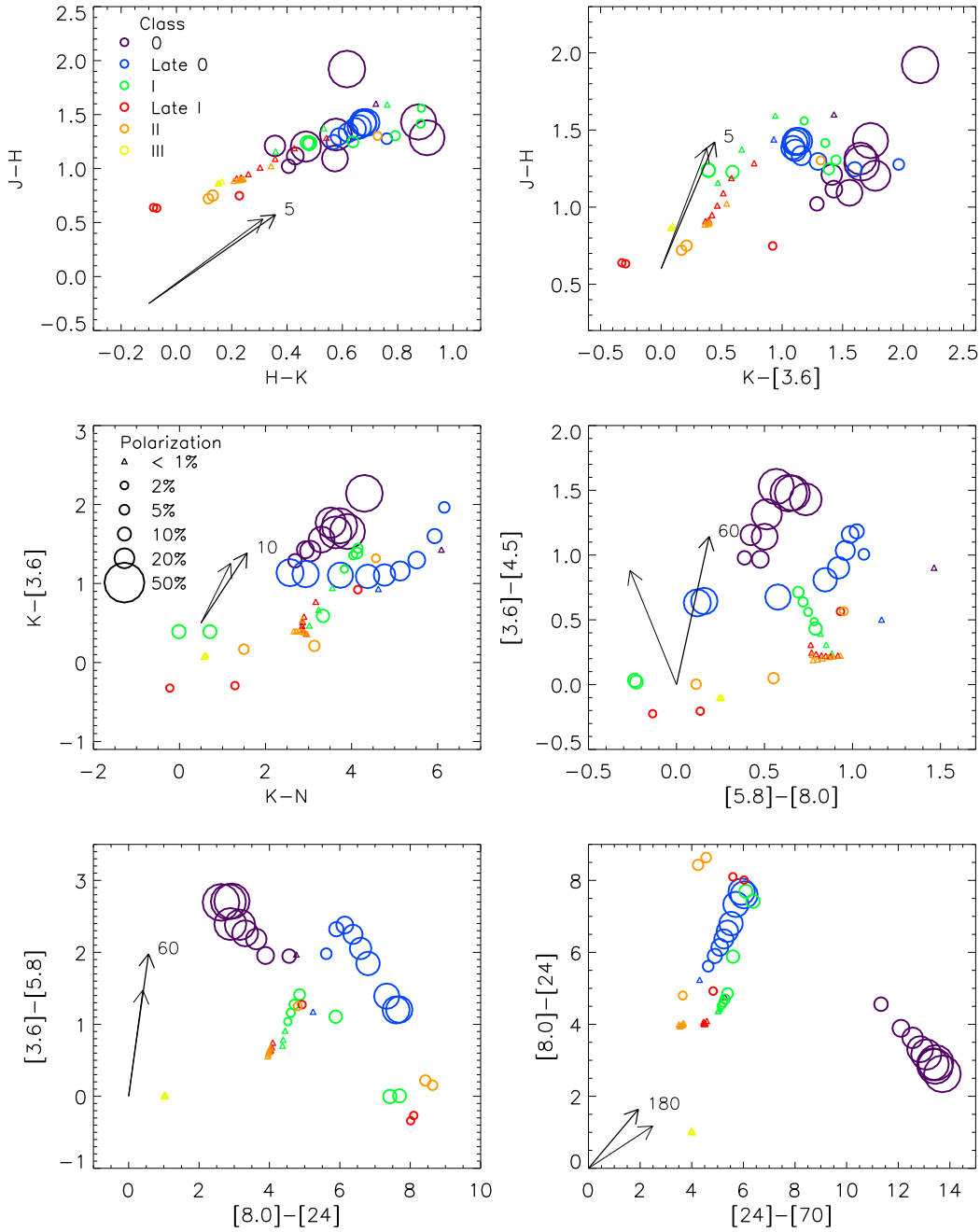
Fig. 10.— Color-color plots showing the large aperture results (5000 AU). This is similar to Figure 7b except that the size of the symbols corresponds to the K-band polarization as shown in the legend in the middle left panel. Points with polarization less than 1% are plotted as small triangles. This shows that near-IR polarization can separate the Class 0 sources from others in the same region of color-color space.
