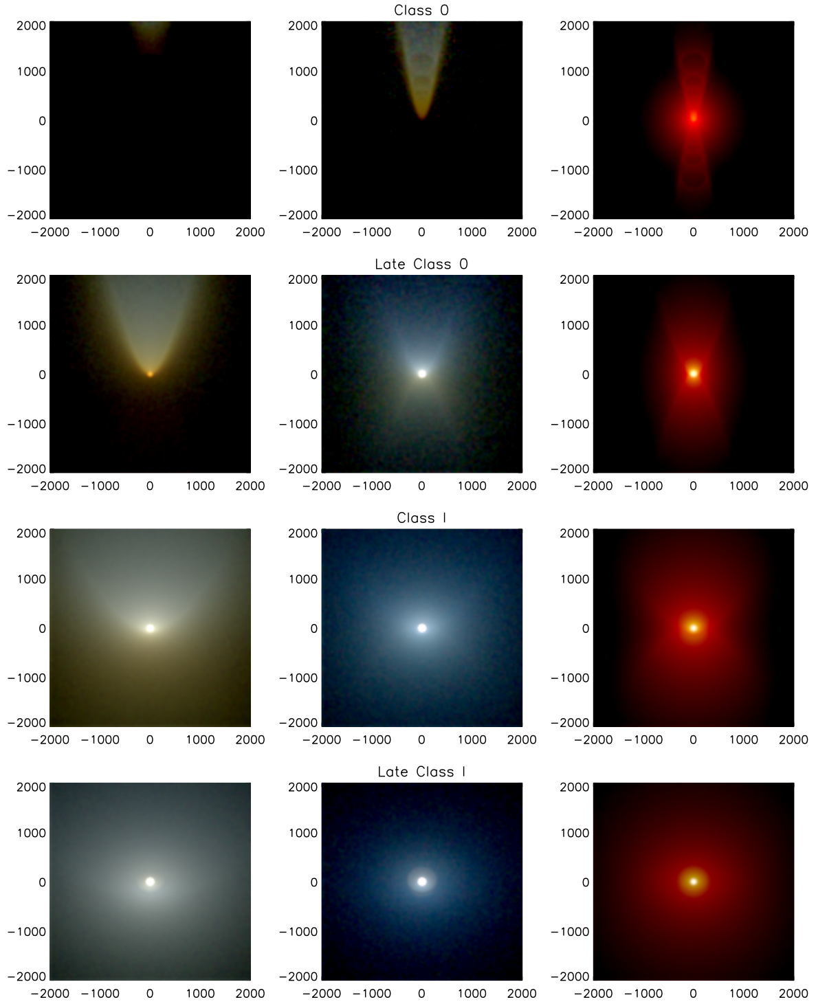
Fig. 12a.— Same as Figure 12 but viewed at a 30°inclination
